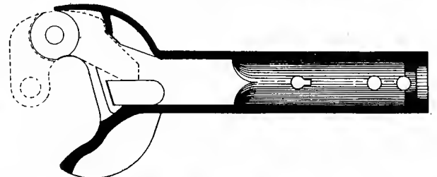
Fig. 2153. Part Section, showing Lock and Knuckle.
